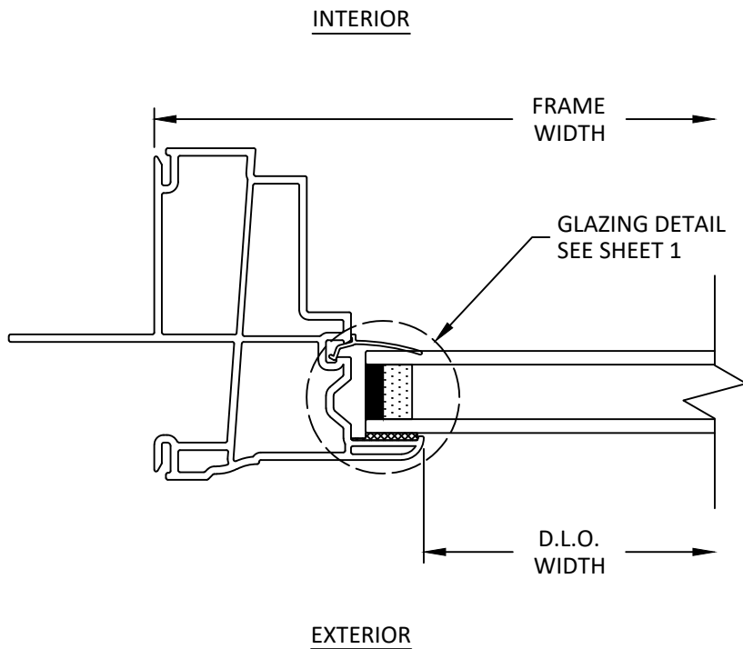
C 4 HORIZONTAL SECTION WINDOW JAMB
