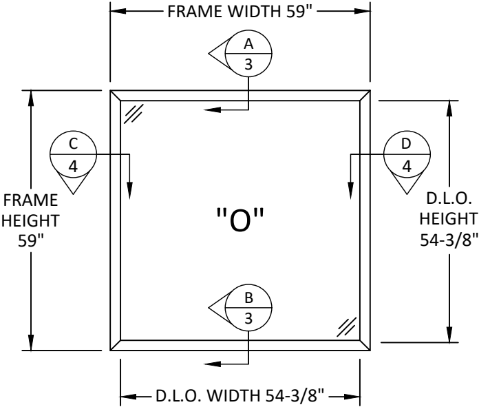
TYPICAL ELEVATION WET GLAZED
