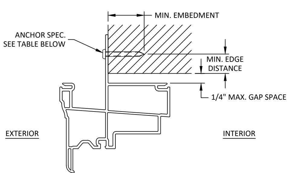
E 5 INSTALLATION DETAIL NAIL FIN HEAD INSTALLATION
