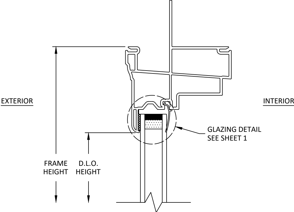
A 3 VERTICAL SECTION WINDOW HEAD
