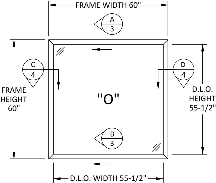
TYPICAL ELEVATION DRY GLAZED
