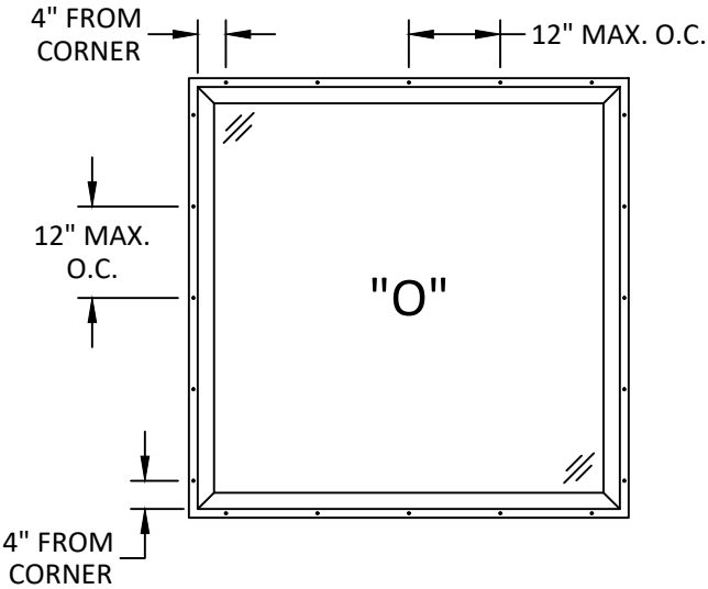
ANCHOR LAYOUT NAIL FIN
