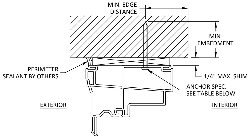
F 5 INSTALLATION DETAIL THROUGH FRAME HEAD INSTALLATION
