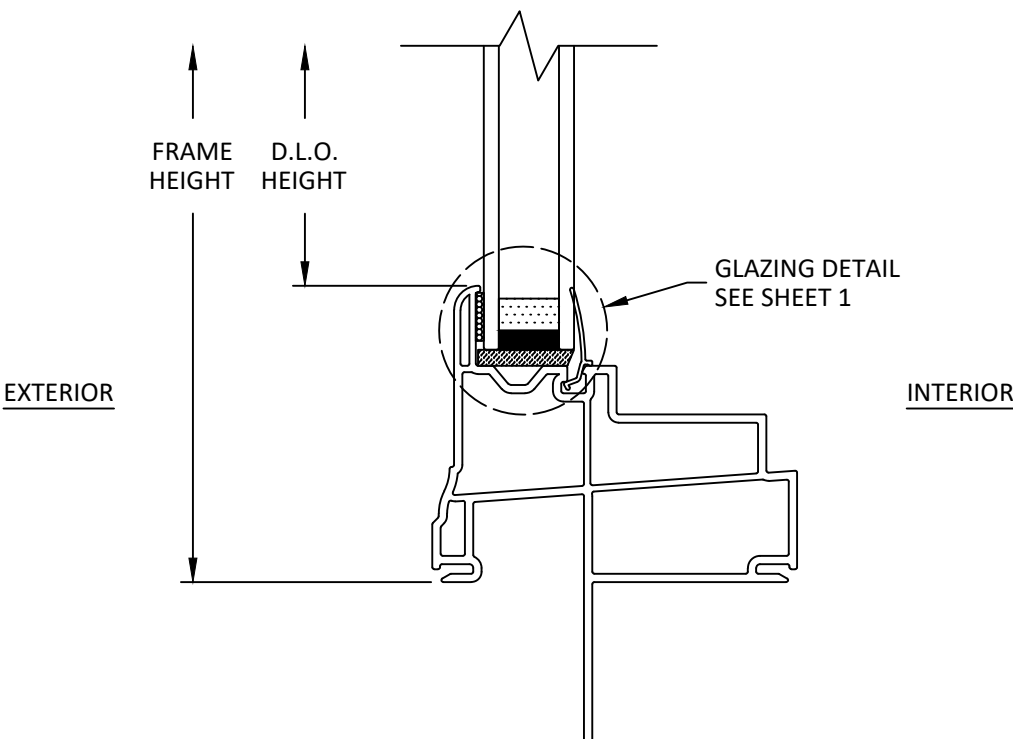
B 3 VERTICAL SECTION WINDOW SILL
