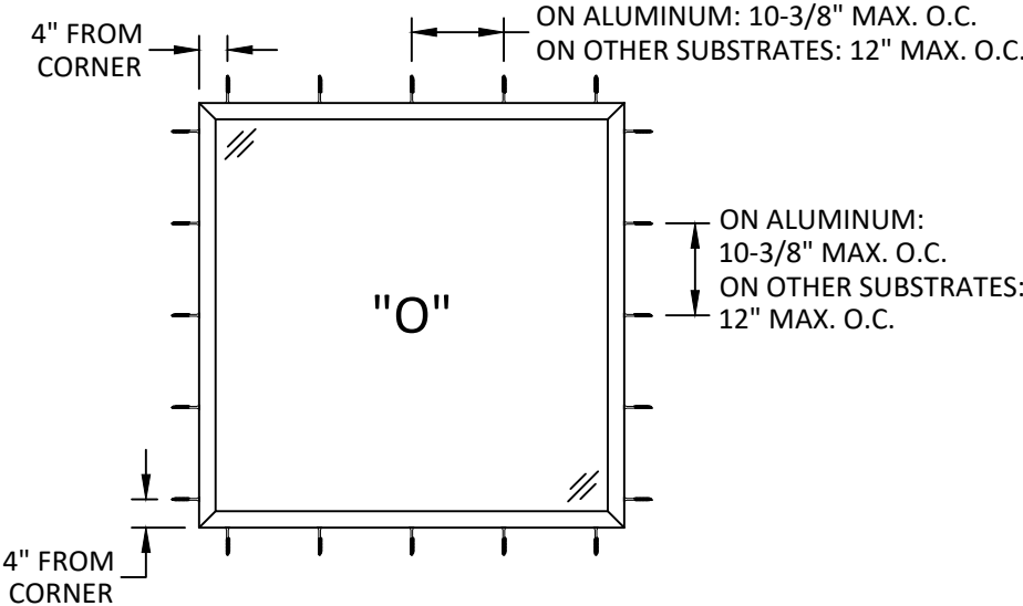
ANCHOR LAYOUT THROUGH FRAME
