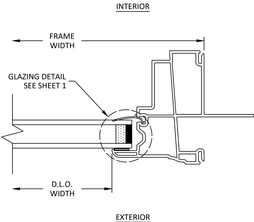
D 4 HORIZONTAL SECTION WINDOW JAMB
